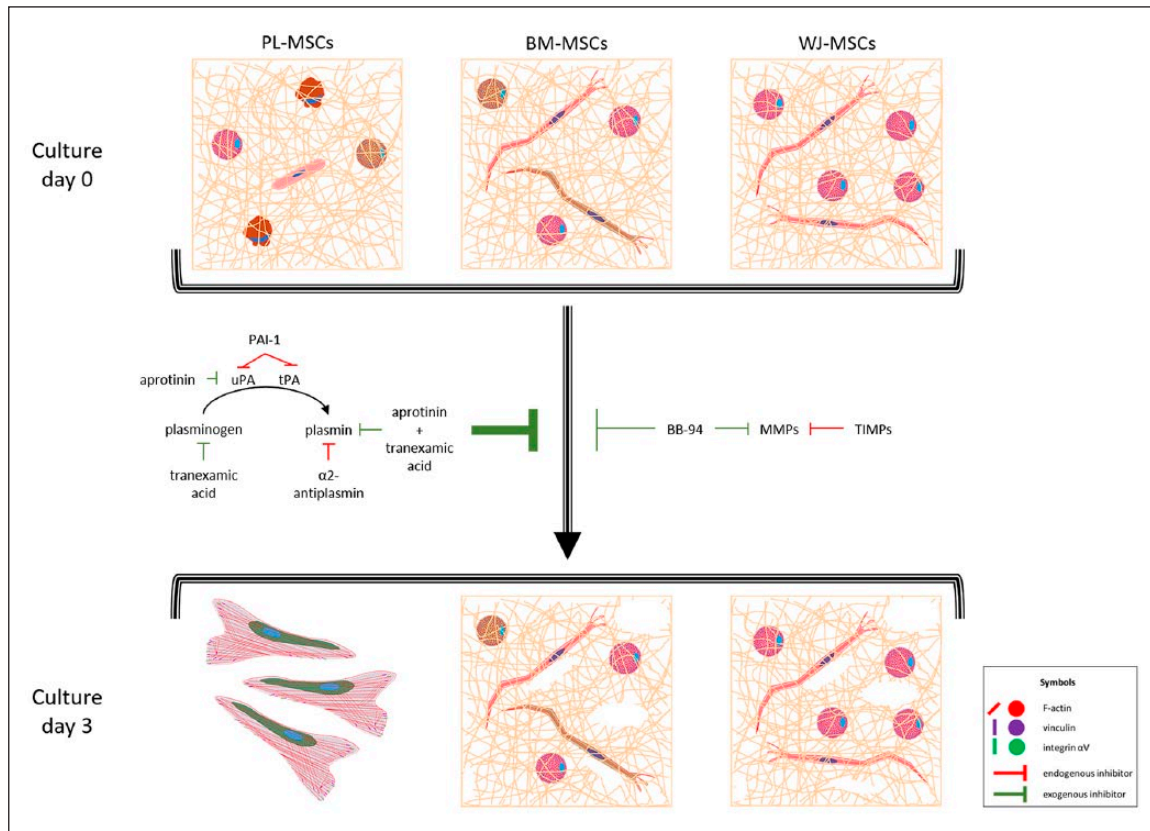
Figure 7. MSCs adhesion to fibrin hydrogels and fibrinolysis effect. MSCs from the three tissues cultured in fibrin hydrogels exhibited elongated and round phenotypes, with actin in filaments or aggregates, respectively. Vinculin and integrin \alpha V were not necessary for adhesion, as they were absent in FAs, and only some cells were positive for both proteins. Proportions of elongated and round-shaped cells varied between the three types of MSCs accordingly to their capabilities to degrade fibrin hydrogel. PL-MSCs were rounded in >90\% , degraded the hydrogel completely, and generated a monolayer with FAs rich in vinculin (see Supplemental Figure S1), and were positive probably for integrin \alpha V (as it was shown in 2D cultures, see Figure 5). BM-MSCs and WJ-MSCs degraded fibrin in a limited way, and after 3 days they still gathered inside it. In all cases, aprotinin and tranexamic acid inhibited fibrinolysis more than BB-94, meaning that it was done principally via the plasminogen–plasmin axis. uPA: urokinase plasminogen activator; tPA: tissue plasminogen activator; PAI-I: plasminogen activator inhibitor I; MMPs: metalloproteases; TIMPs: tissue inhibitors of metalloproteases.
